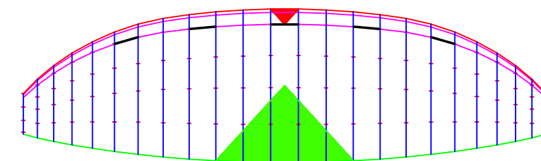
BHL-S 20 m 2 23 panels span=9.18 m AR=4.2
