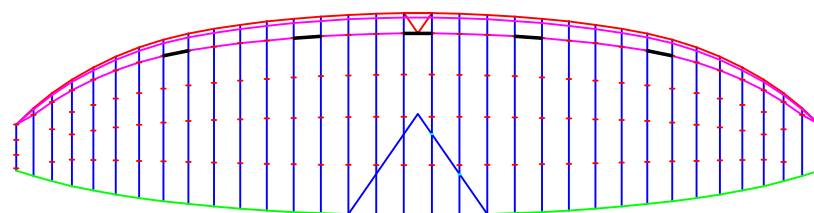
BHL2 19 m 2 33 panels span=9.71 m AR=5.0
