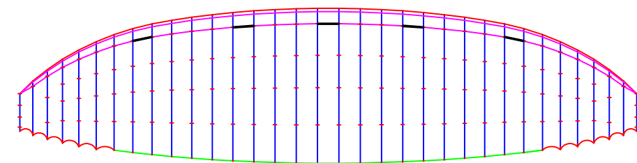
BHL2 23 m 2 "JPS" 33 panels span=10.7 m AR=5.0
