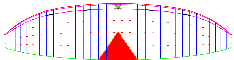
BHL2 23 m 2 33 panels span=10.69 m AR=5.0
