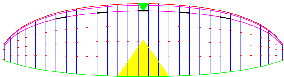
BHL & JAP 25 m 2 29 panels span=10.84 m AR=4.7
