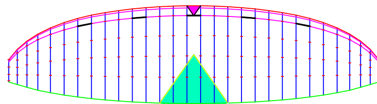
BHL 18 m 2 29 panels span=9.20 m AR=4.7
